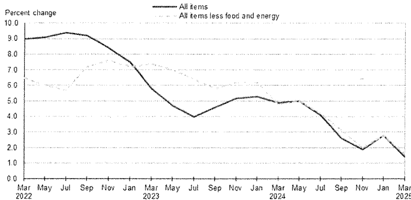
Chart 1. Over-the-year percent change in CPI-U, Dallas-Fort Worth-Arlington, TX, March 2022–March 2025
