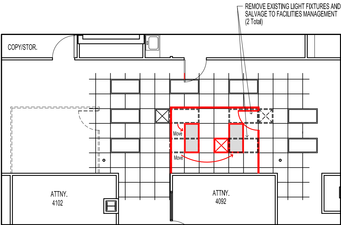
FLOOR PLAN - AREA A
